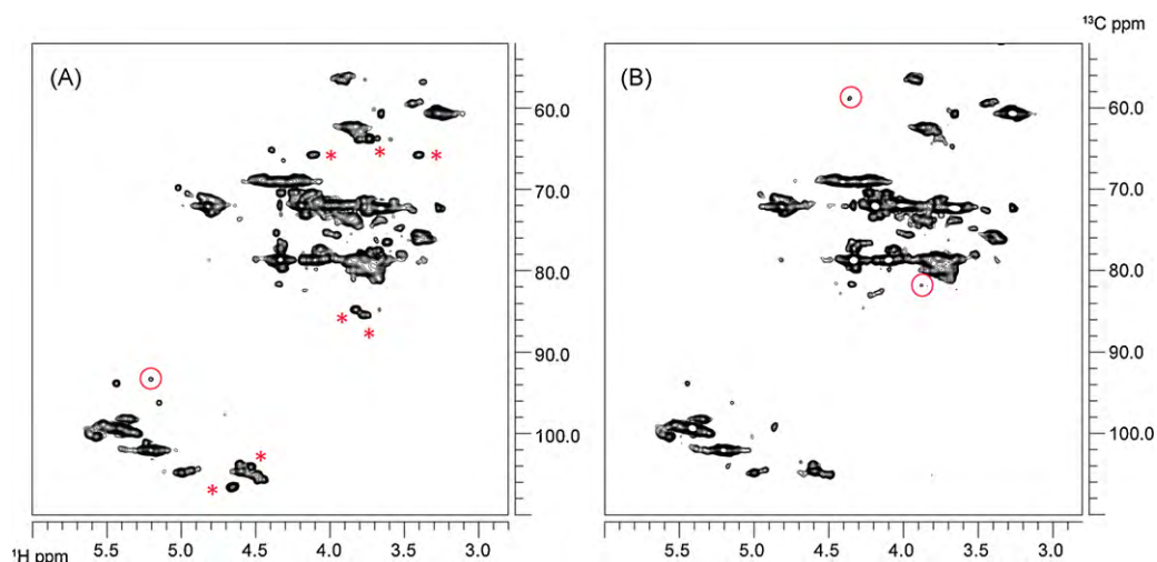
Fig. 6. (A) HSQC spectrum of UFH heparin lot 2. The H1/C1 signal of GlcNAc \alpha reducing end is circled. (B) HSQC spectrum of UFH heparin lot 2 treated with \text{KMnO}_4 . The H1/C1 signal of GlcNAc \alpha reducing end disappeared, while signals at 4.37/58.9 and 3.88/81.8 ppm appeared (see circled signals). Signals due to the linkage region (indicated with * in A) are also missing.
