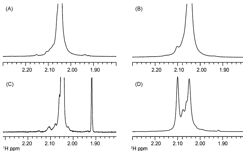
Fig. 2. ^1\text{H} NMR spectra of (A) PI-HS, (B) PI-HS ox , (C) PI-HSNac and (D) PI-HSNac ox . Only the N -acetyl region of the spectra is shown. The signal at 1.92 ppm is due to acetate salt.
