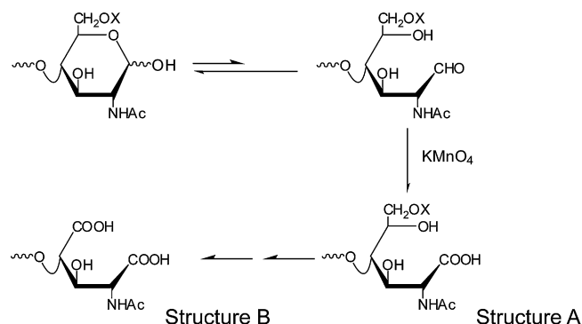
Fig. 7. Reaction scheme outlining the formation of Structure A ( N -acetylglucosaminic acid; where X = H or \text{SO}_3 ) generated as a result of potassium permanganate oxidation at the reducing end of chains. It is possible that further oxidation of Structure A (if X = H) may result in the formation of a dicarboxylic acid (Structure B). However, Structure B is a proposed structure, and no confirmation of this structure is provided at present.
