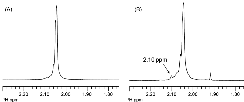
Fig. 1. 1 H NMR spectra of (A) unfractionated heparin lot 2. The signal at 2.10 ppm is absent. (B) Unfractionated heparin lot 1. The signal at 2.10 ppm is labeled. The signal at 1.92 ppm is due to acetate salt.
