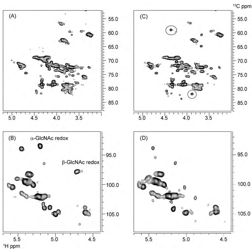
Fig. 3. HSQC spectrum of PI-HSNAC: (A) non-anomeric region and (B) anomeric region. Signals due to H1/C1 GlcNAc \alpha and \beta reducing ends, are indicated. HSQC spectrum of PI-HSNAC ox : (C) non-anomeric region (the cross peaks at 4.37/58.9 ppm and 3.88/81.8 ppm are circled), and (D) anomeric region.
