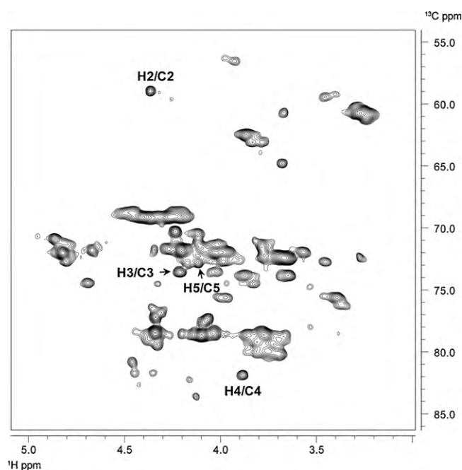
Fig. 5. HSQC spectrum of PI-HSNAC ox . NMR assignments for the oxidized residue are indicated close to the relative contours.
