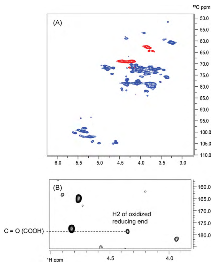
Fig. 4. (A) HSQC-DEPT spectrum of PI-HSNAC ox . CH cross peaks are indicated in blue, CH 2 cross peaks are indicated in red. The cross peak at 4.37/58.9 ppm is circled. (B) HMBC spectrum of PI-HSNAC ox . The long-range correlation between the proton at 4.37 ppm and a carbonyl group is indicated.
